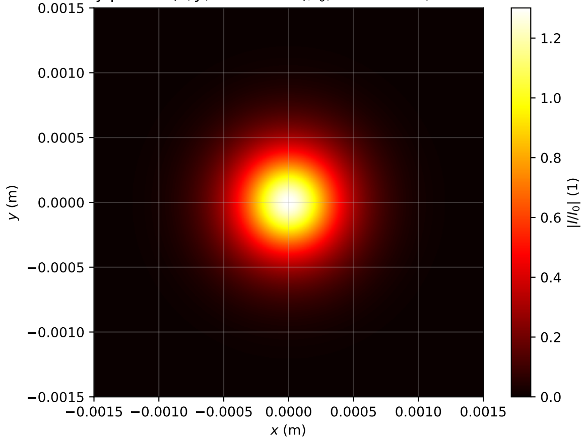
Intensity profile I(x, y, z = 0.796m)/I_0 , Pin=0.9Pcr, artificial time
